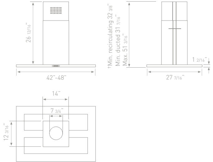
*Ductless (recirculating); louver holes exposed. Note: if necessary order the proper duct cover extension kit.
